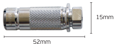
UC-2121 ULTRAFLO Quick Release Grease Coupler
